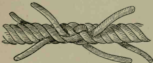
FIG. 106 D.—Short splice (continued).
